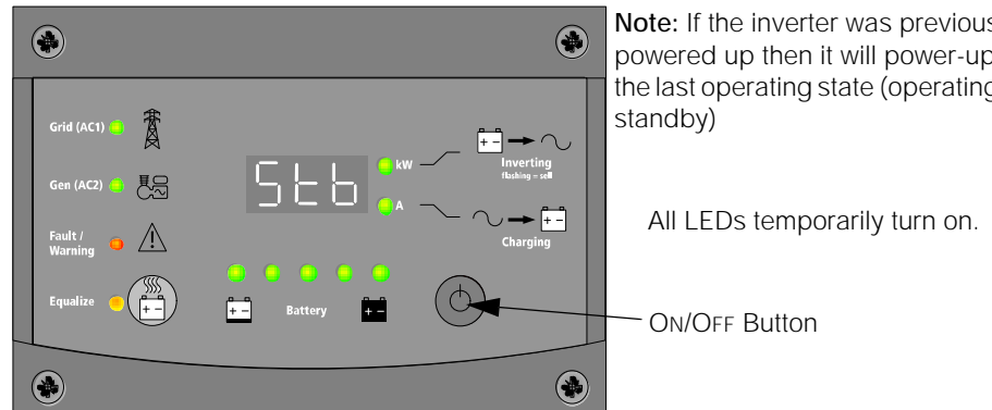
Figure 2-22 Power-up Display
