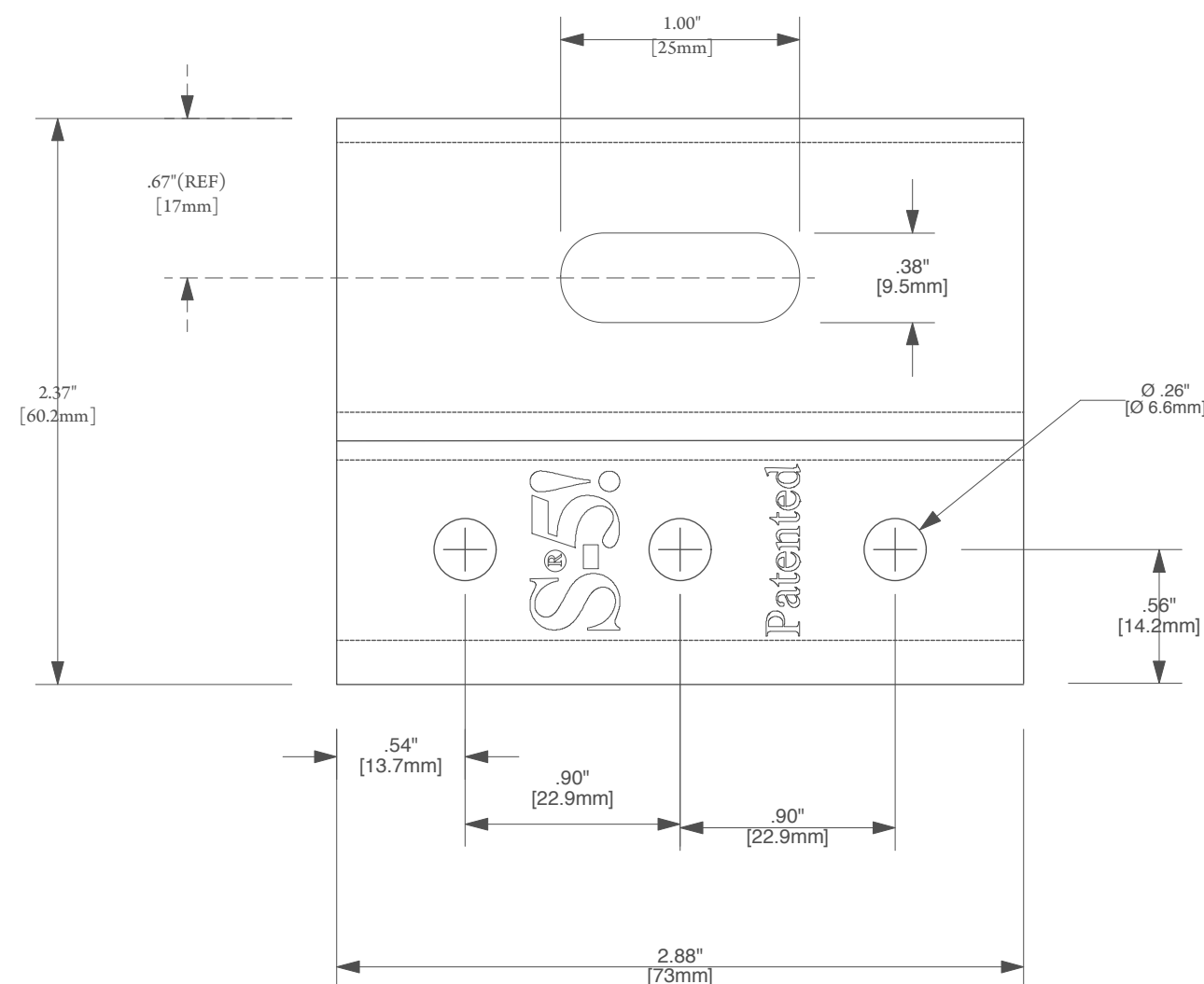
TOP VIEW
