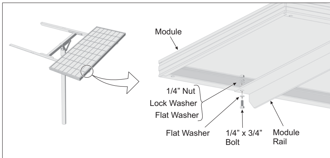
Figure 4-1: Installing PV Modules to Module Rails
