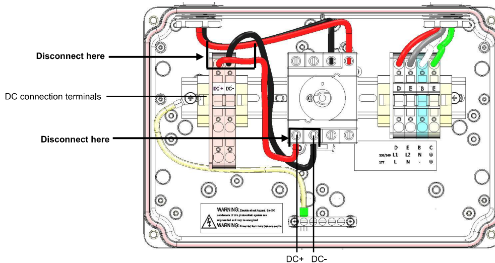
Figure 3: Three-phase inverter Safety Switch with DC terminal blocks
