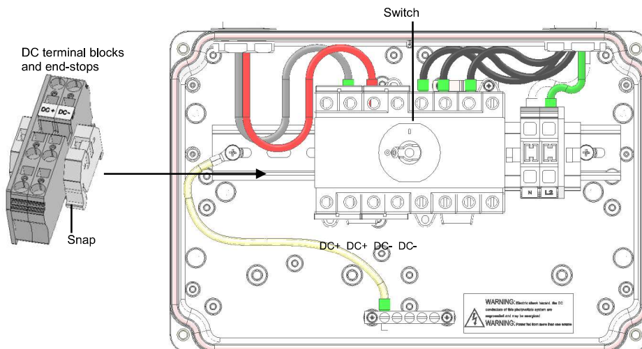
Figure 1: Three-phase inverter Safety Switch without DC terminal blocks
