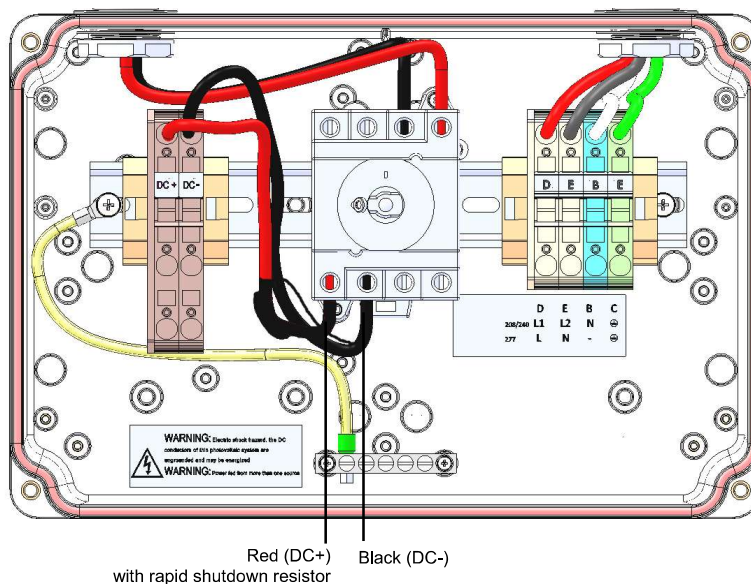
Figure 4: Three-phase inverter Safety Switch – connecting the Rapid Shutdown cable
