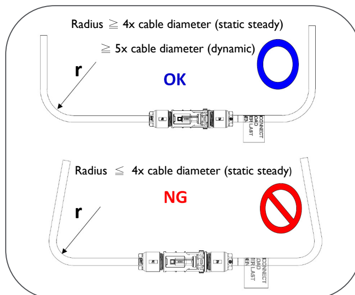
Fig. 5 Minimum bending radius of cable
