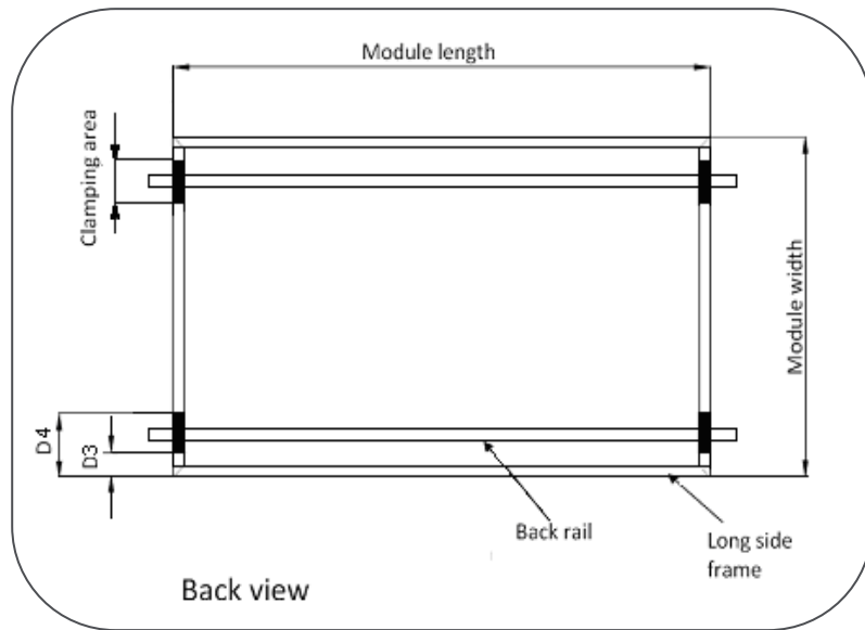
Figure 4 Effective mounting area (clamping )
