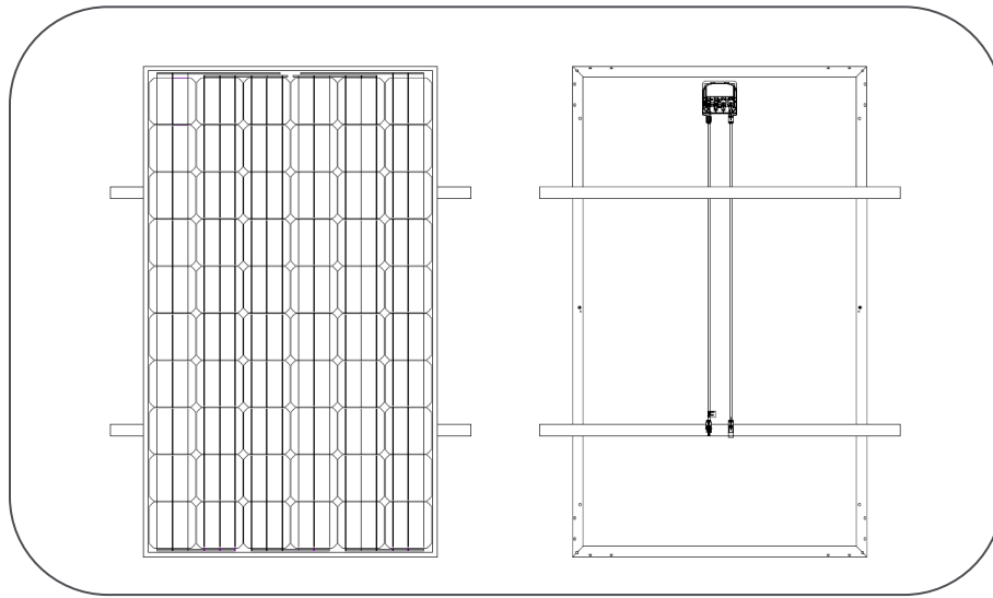
Figure 2 Installation of module
