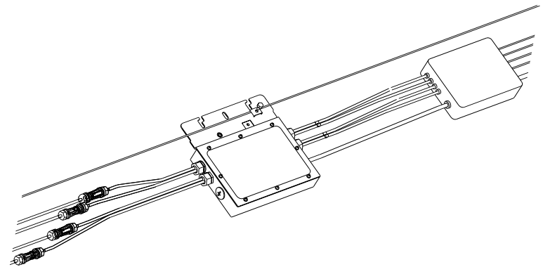
▲ Figure 3.6 Ground connection
