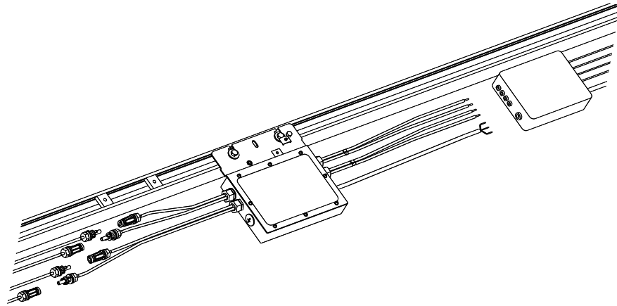
▲ Figure 3.3 Fix the screws
