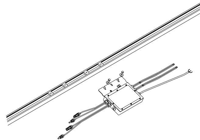
▲ Figure 3.2 Attaching RSD to rack
