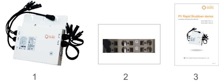
▲ Figure 1.3 Parts
