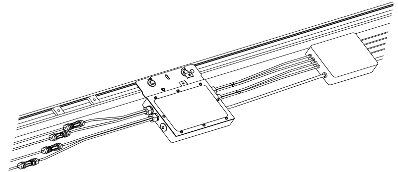
▲ Figure 3.4 Connect DC input connectors
