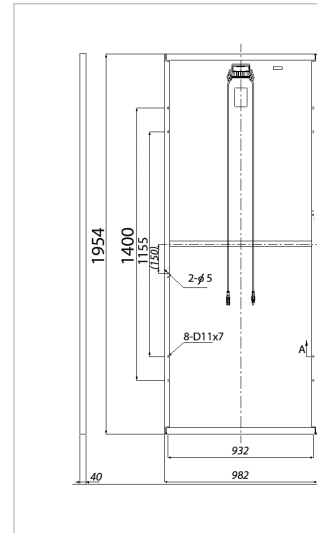
Rear View
