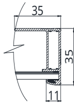
Frame Cross Section A-A
