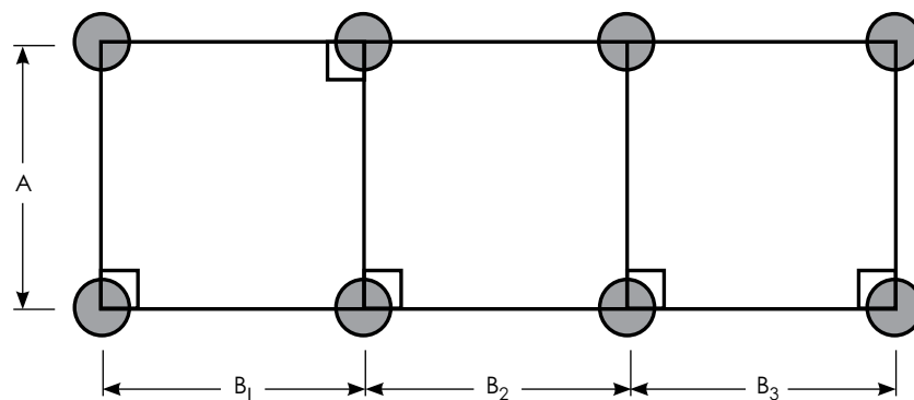
Figure 5. North-south leg spacing is fixed and listed on your Specs Sheet (Specific Values under “Design Parameters,” p. 2). East-west spacing ( B_1 , B_2 , etc.) is identical in most installations; see “Average leg spacing e-w” (Nominal Values under “Design Parameters”) on page 2 of your Specs Sheet. However, if you needed to shift leg positions, follow the east-west spacing you set during your planning session.
